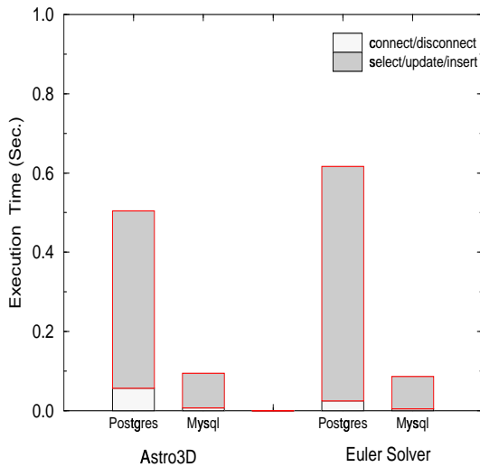
Figure 7: Cost of accessing the database for the two applications
