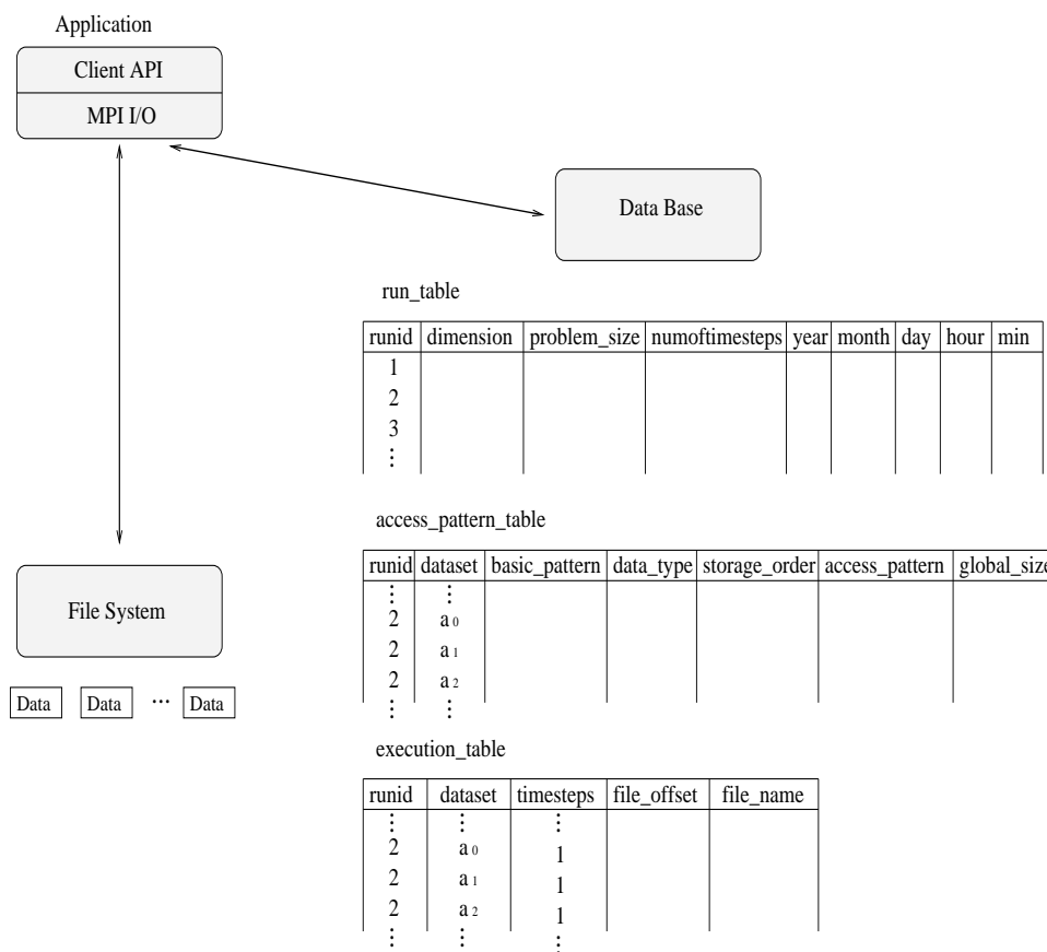
Figure 2: Database tables used in SDM
