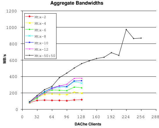
Figure 4. The number of clients at which bandwidth knees over is dependent on how many lock servers there are.
